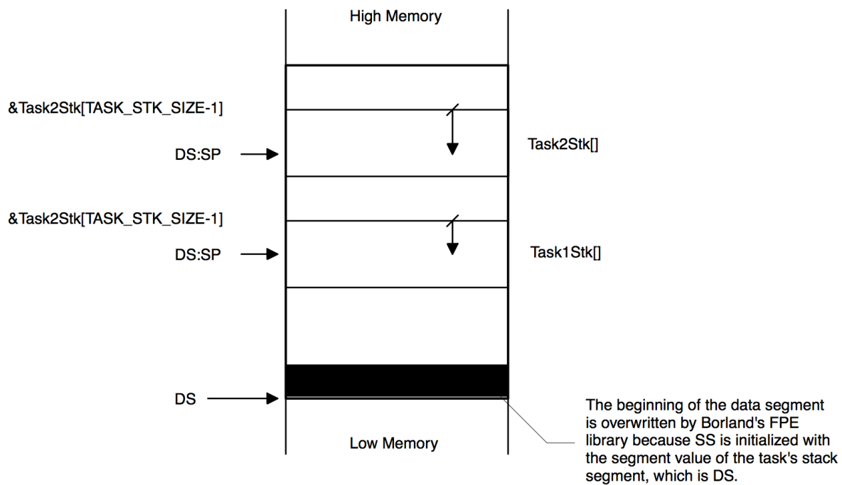
Figure - Figure 14.5 Borland Floating-Point emulation stack.
