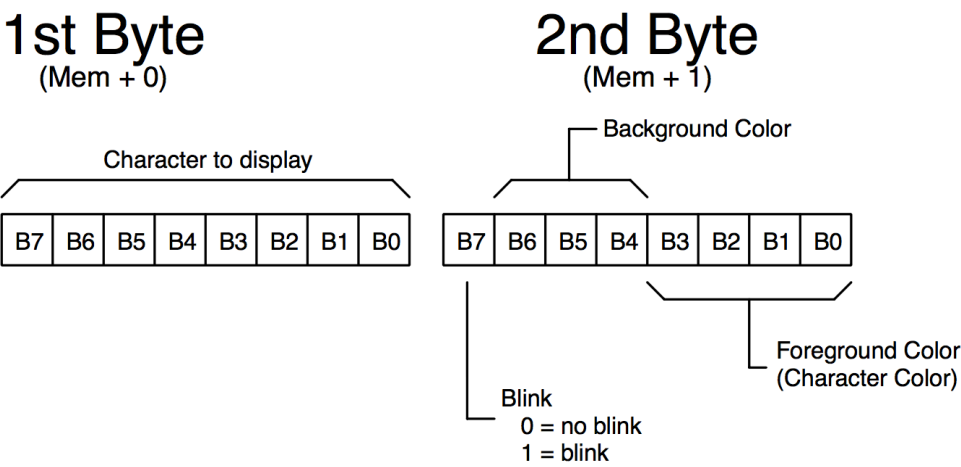
Figure - Figure 20-2, Character and attribute bytes on a VGA monitor
