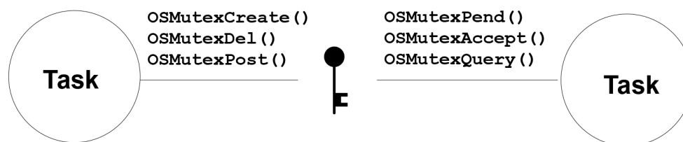
Figure - Figure 8.1, Relationship between tasks and a mutex
