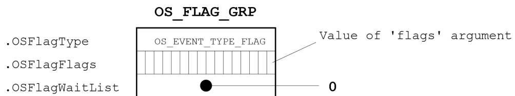
Figure - Figure 9.3 Event Flag group just before OSFlagCreate() returns
