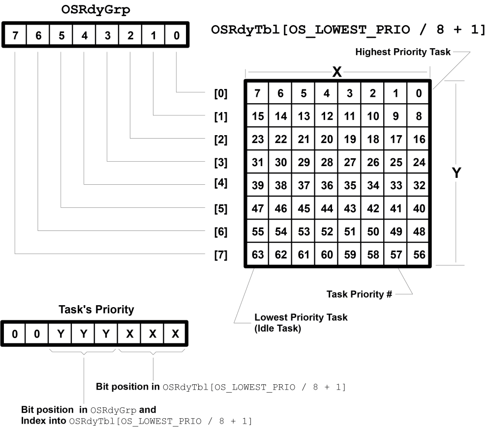
Figure - Figure 3.4 The µC/OS-II ready list
