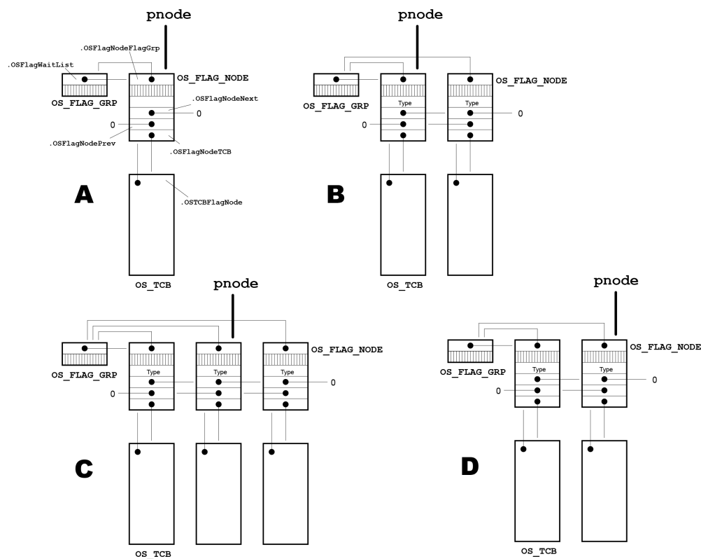
Figure - Figure 9.5, Removing an OS_FLAG_NODE from the wait list
