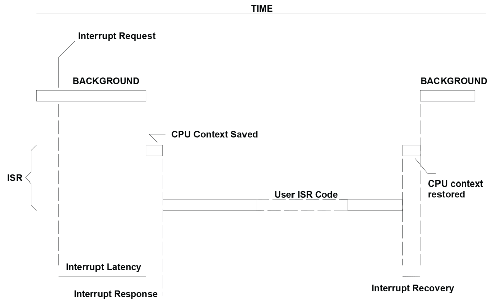
Figure - Figure 2.20 Interrupt latency, response, and recovery (foreground/background)
