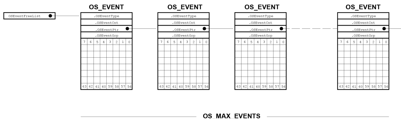
Figure - Figure 6.5 List of free ECBs
