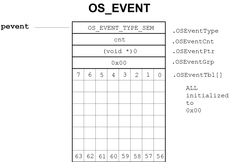
Figure - Figure 7.2 ECB just before OS_SemCreate() returns
