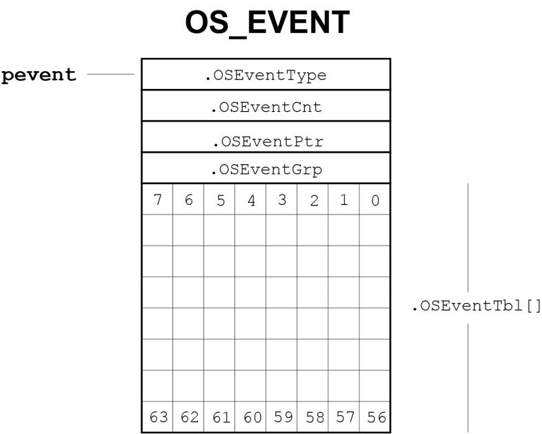
Figure - Figure 6.2, Event Control Block (ECB)
