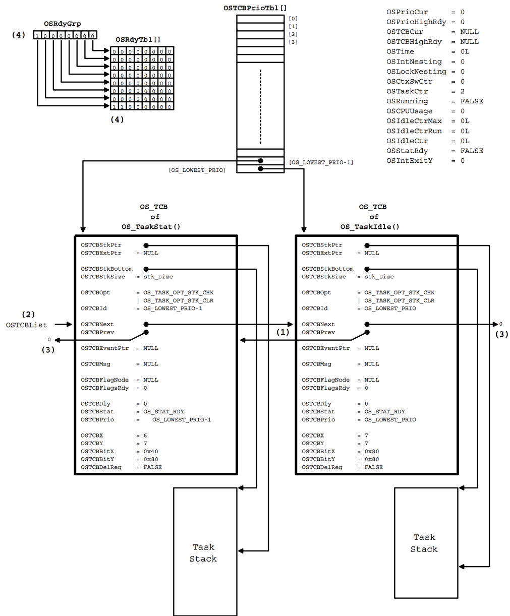
Figure - Figure 3.11 Variables and Data structures after calling OSInit()
