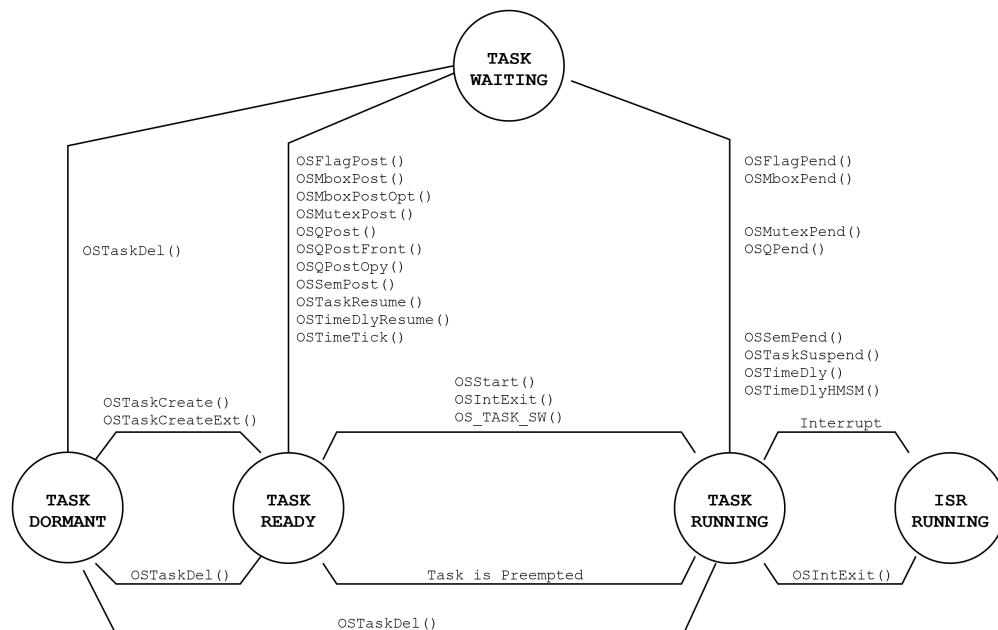
Figure - Figure 3.2 Task states
