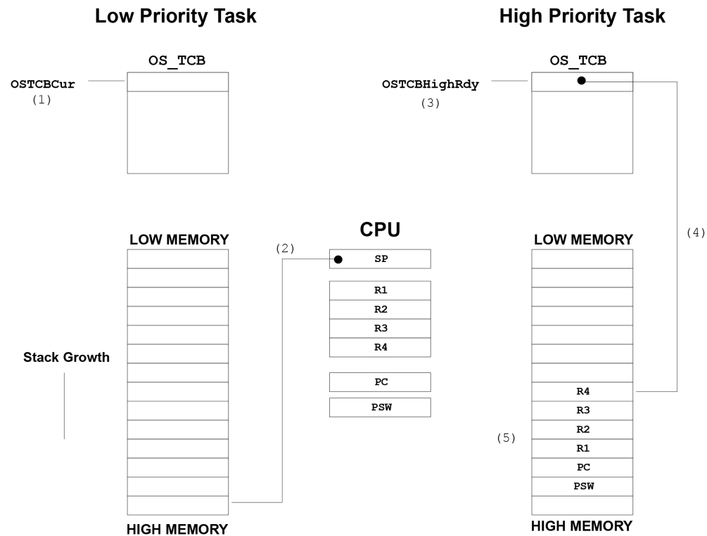
Figure - Figure 3.6 µC/OS-II structures when OS_TASK_SW() is called
